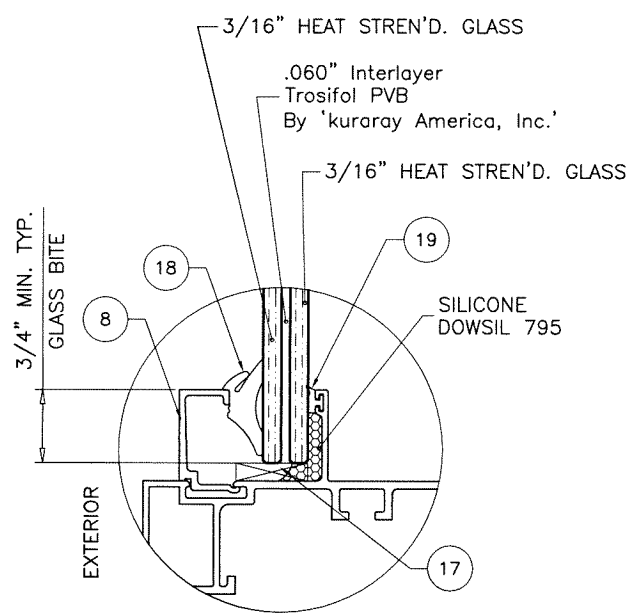
GLAZING DETAIL FIXED WINDOW 7/16" NOMINAL OVERALL LAM. GLASS
